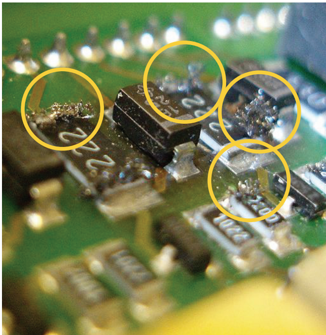
Figure 1 – The Restriction of Hazardous Substances (RoHS) directive, which originated in the European Union, restricts dangerous substances commonly used in electronics. The photograph above shows silver whiskers growing out of RoHS compliant circuit board components
